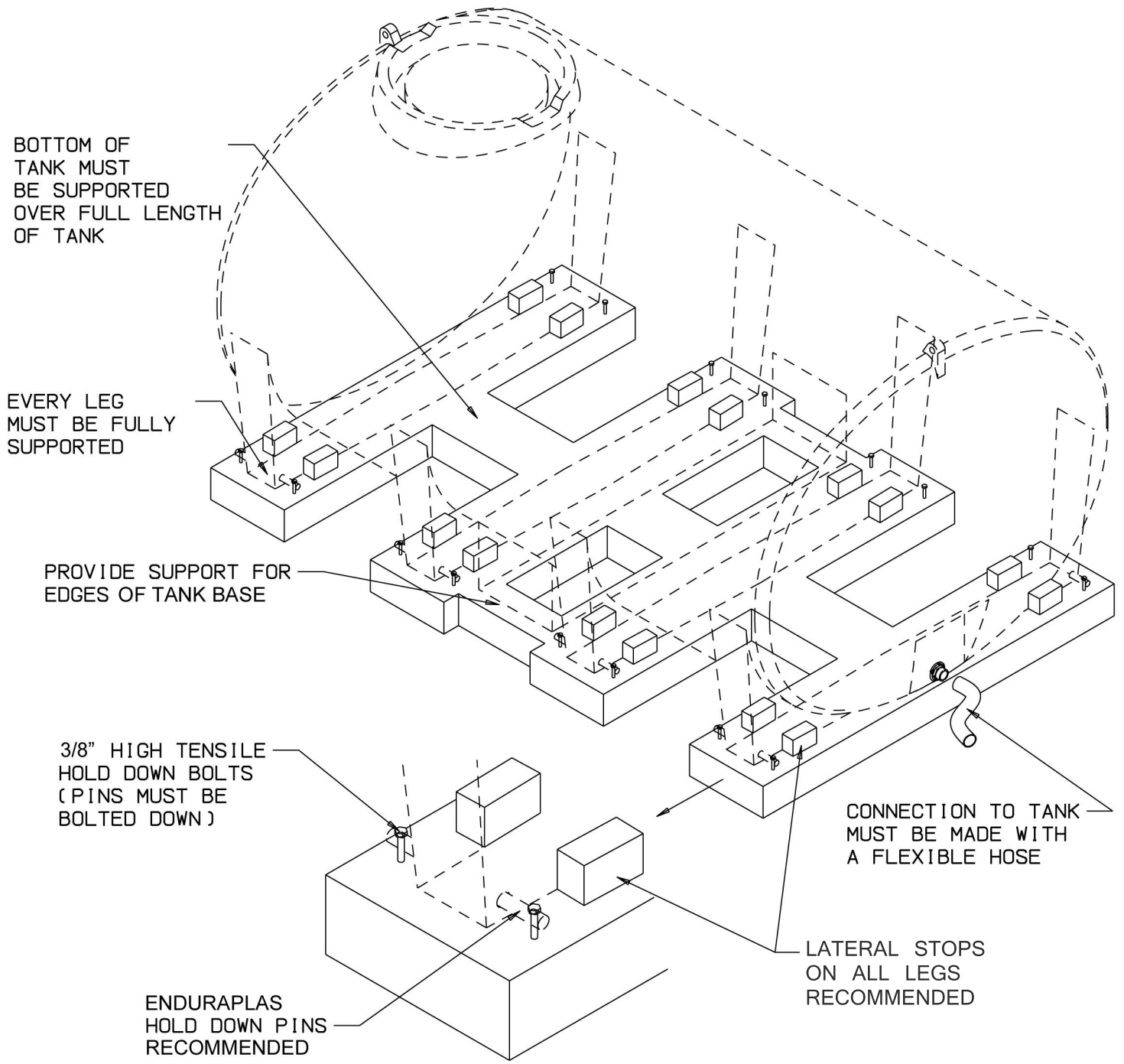
ENLARGED TYPICAL DETAIL
